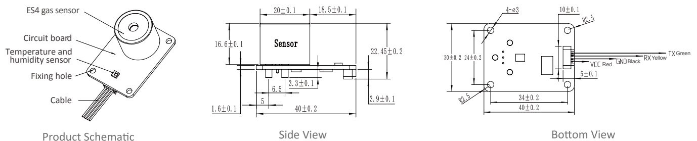
TB200B-ES4-CH 4 S Dimension diagram
