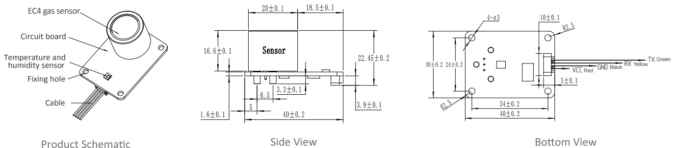
TB200B-EC4-Br 2 Dimension diagram
