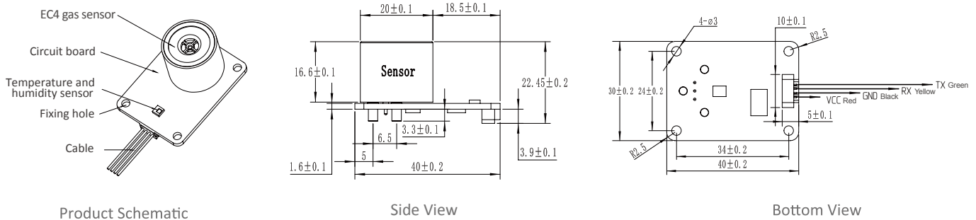
TB200B-EC4-Cl 2 Dimension diagram
