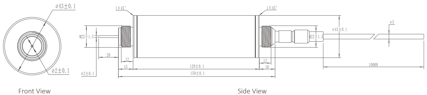
05-ECtox-HT-NH 3 -500-01 Dimension Diagram
