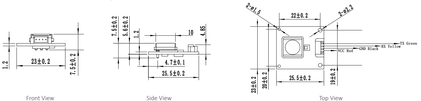
TB600B-WQ-HCHO-1 Dimension diagram
