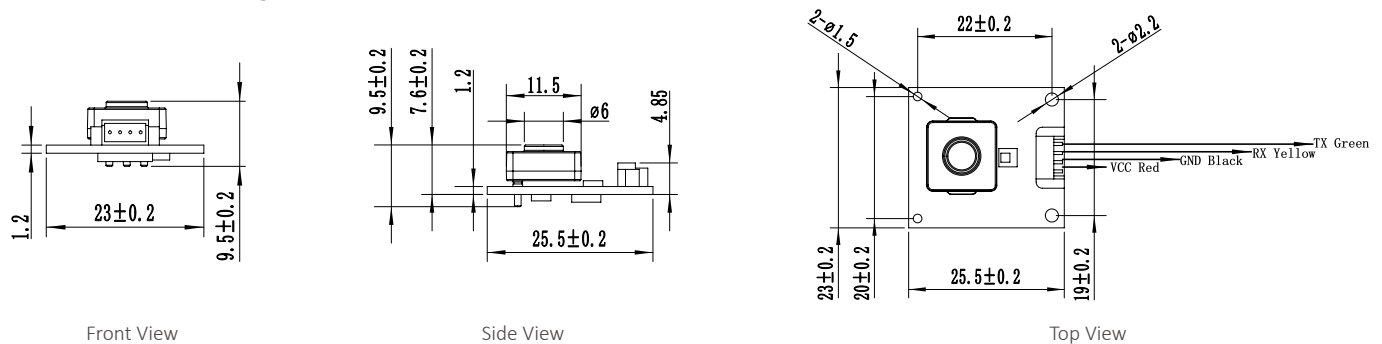
TB600B&amp;C Dimension diagram
