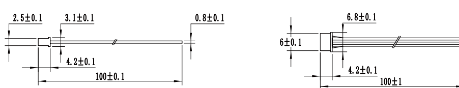
4pin Cable Diagram
