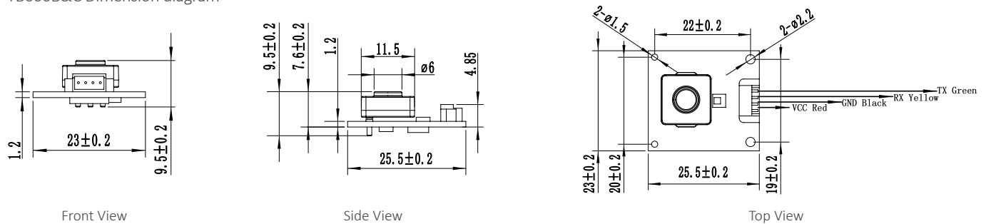
TB600B&amp;C Dimension diagram
