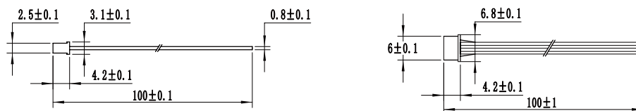
4pin Cable Diagram
