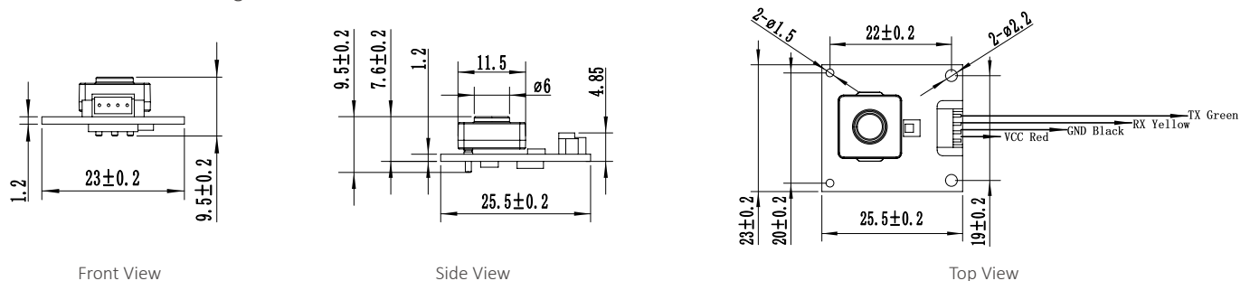
TB600B&C Dimension diagram
