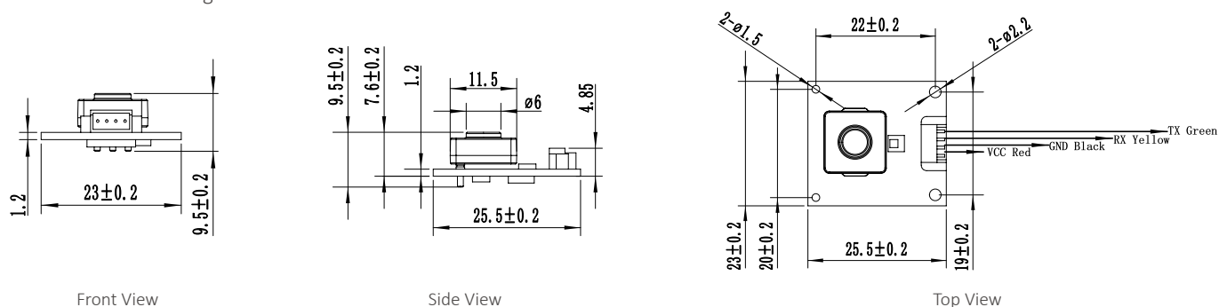
TB600B Dimension diagram
